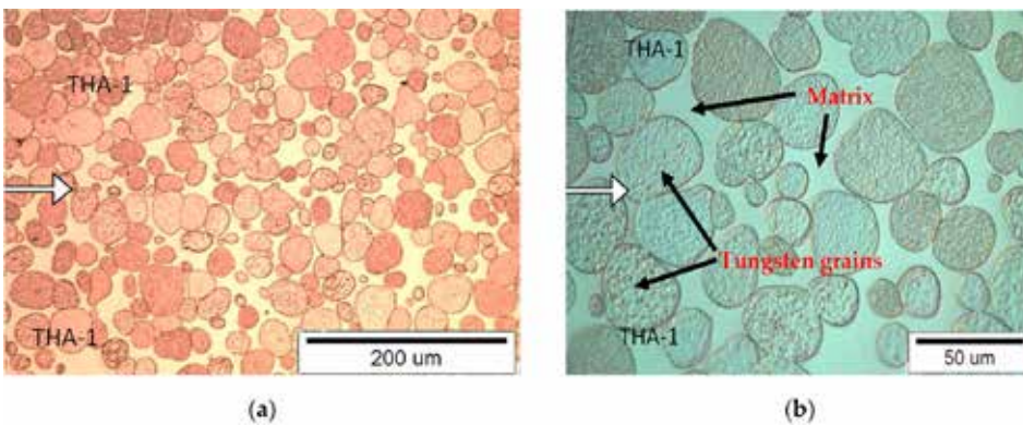
Figure 3: View of the microstructure of the THA-1 with THA-1 at a magnification of 200× (a) and 500× (b), [the connection line (joint) is shown by the arrow].
