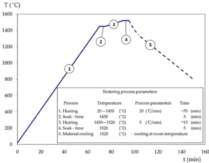
Figure 2: Join-process temperature diagram.
