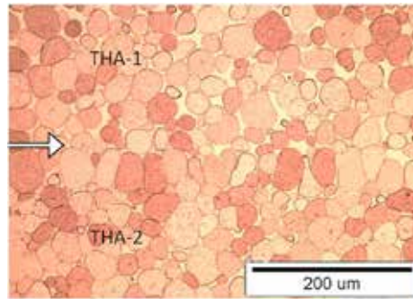
Figure 7: View of the microstructure of the THA-1 with THA-2 (with THA-1 on the top) at a magnification of 200× (a) and 500× (b), [the connection line (joint) is shown by the arrow].
