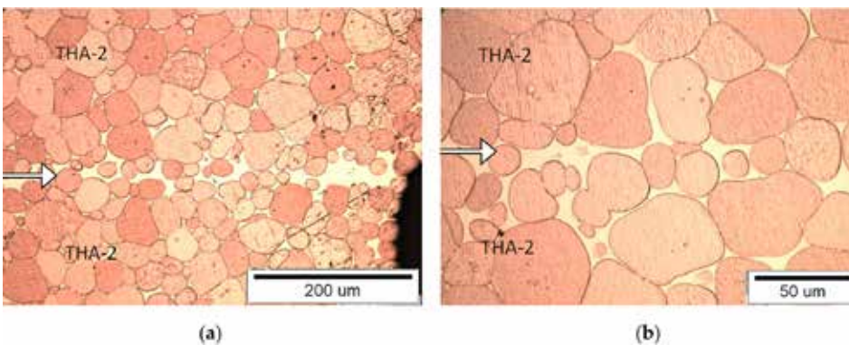
Figure 4: View of the microstructure of the THA-2 with THA-2 at a magnification of 200× (a) and 500× (b), [the connection line (joint) is shown by the arrow].
