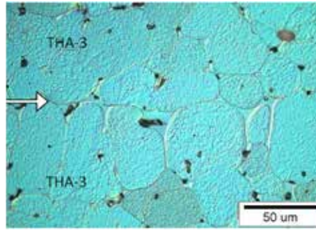
Figure 5: View of the microstructure of the THA-3 with THA-3 at a magnification 500× [the connection line (joint) is shown by the arrow].
